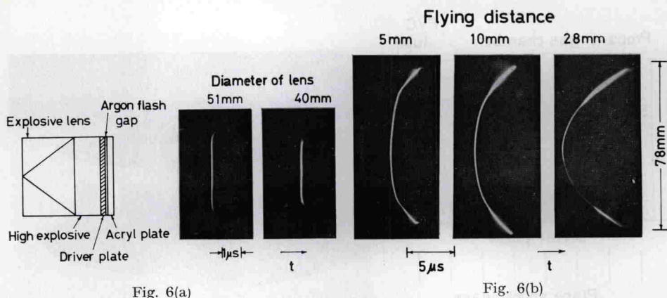
Fig. 6. Planarity of the plane shock wave generators (a) In-contact method (b) Flyer method The flyer plate 78 mm in diameter and 3 mm thick is propelled by 30 mm thick Pentolite pad
